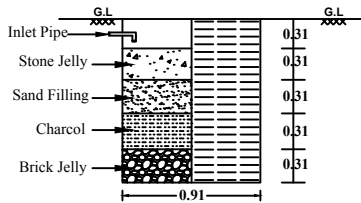
RAIN WATER HARVESTING DETAIL (NOT TO SCALE)
