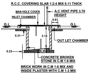
SECTION ON SEPTIC TANK. (NOT TO SCALE)
