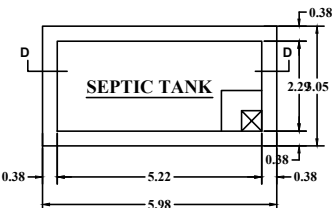
PLAN ON SEPTIC TANK. (NOT TO SCALE)
