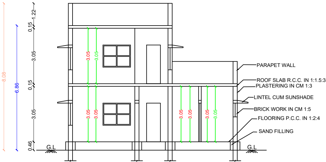
SECTION"A-B"
