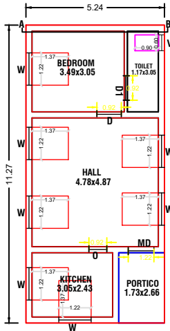
PRO., GROUND FLOOR PLAN
