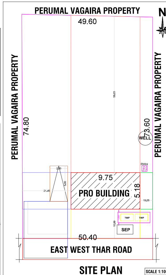
COMPOUND WALL PLAN PERCOLATION PIT
