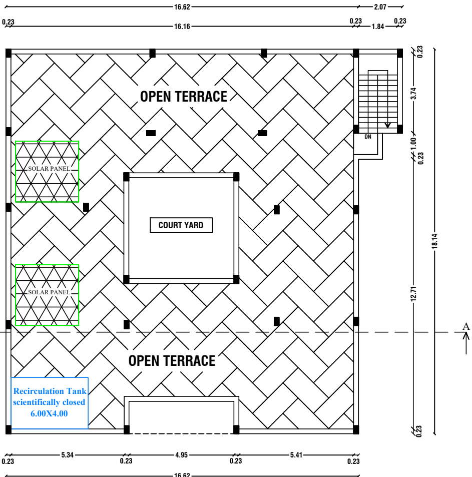
FLOOR - TERRACE PRO. TERRACE FLOOR PLAN
