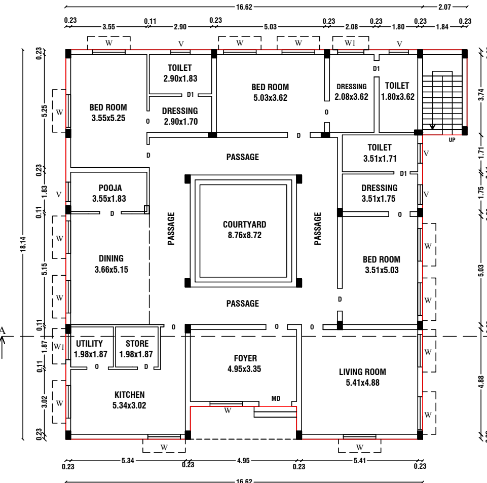
FLOOR - GROUND PRO. GROUND FLOOR PLAN
