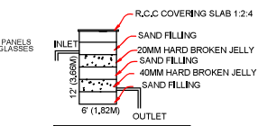
R.C.C. COVERING SLAB 1:2:4
