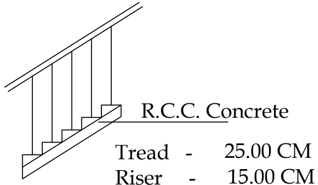
Staircase details
