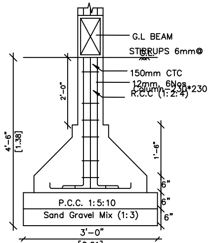
R.C.C. COLUMN FOOTING DETAILS SCALE : 1:25
