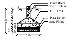
COLUMN FOOTING DETAILS
