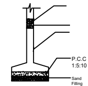
FOUNDATION DETAILS
