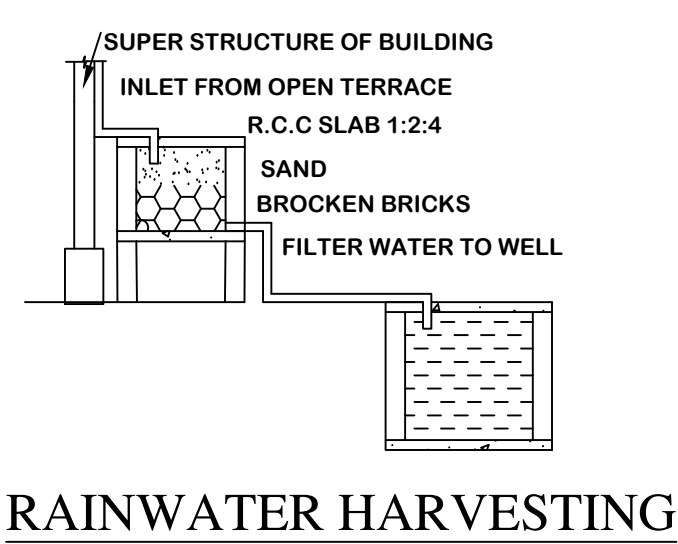
RAINWATER HARVESTING
