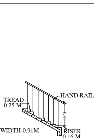
STAIRCASE DETAILS
