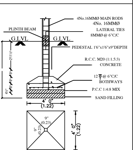
FOUNDATION DETAIL
