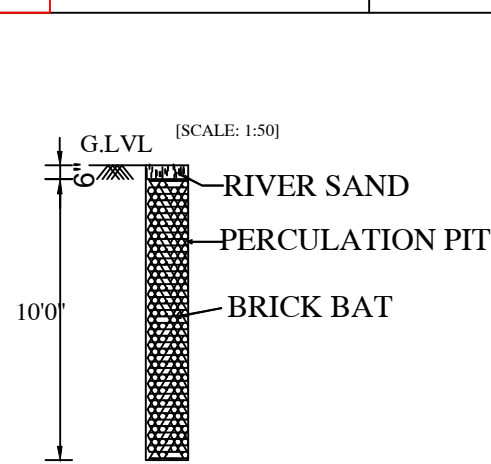
PERCOLATION PIT
