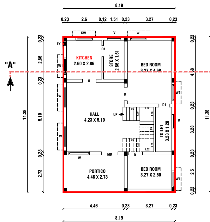
FLOOR - GROUND
