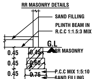
RR MASONRY DETAILS
