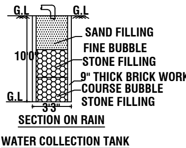
SECTION ON RAIN WATER COLLECTION TANK
