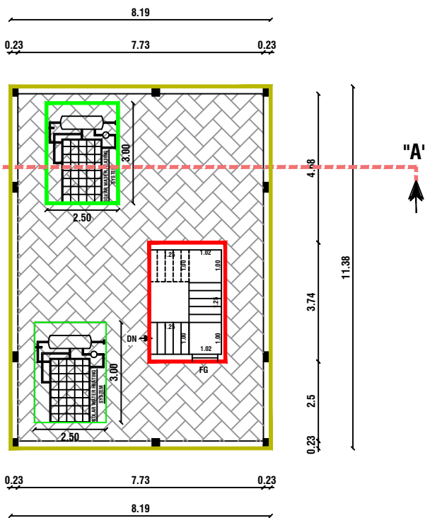
FLOOR - TERRACE
