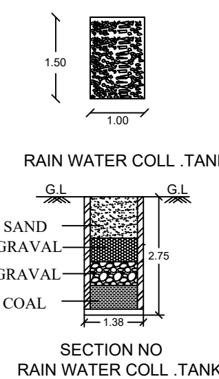
SECTION NO RAIN WATER COLL .TANK
