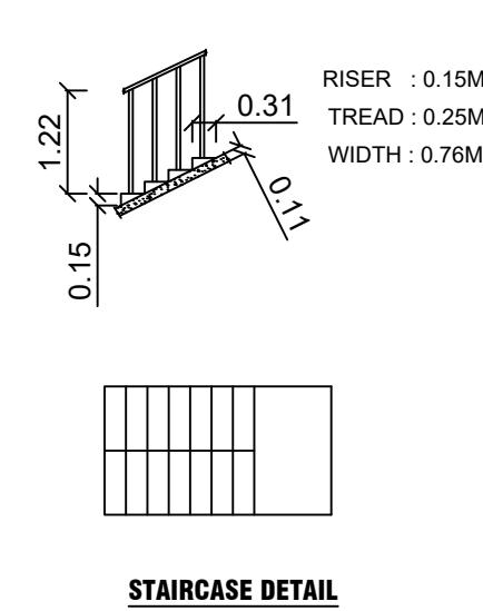
STAIRCASE DETAIL
