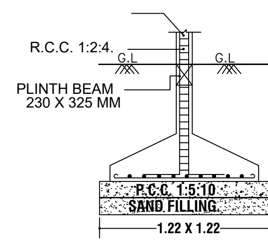
FOUNDATION DETAIL (NOT TO SCALE)
