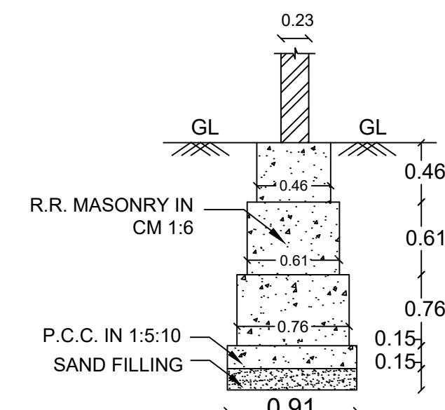
FOOTING DETAIL (NOT TO SCALE)
