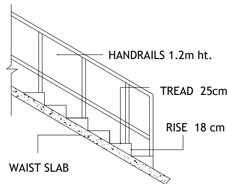
STAIRCASE DETAILS
