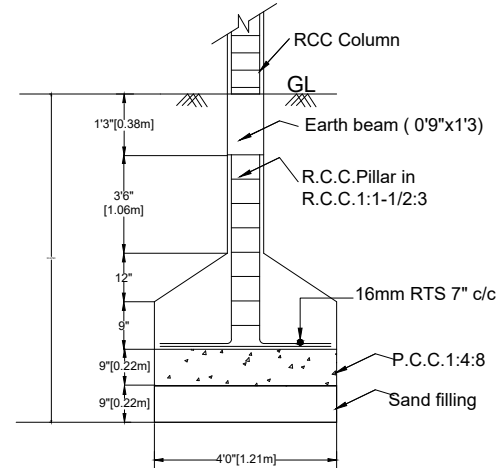
FOUNDATION DETAILS
