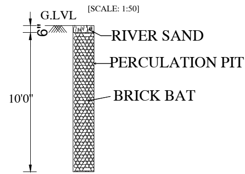
PERCOLATION PIT
