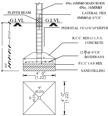
FOUNDATION DETAIL
