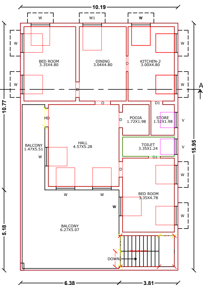
FLOOR - FIRST PRO. FIRST FLOOR PLAN
