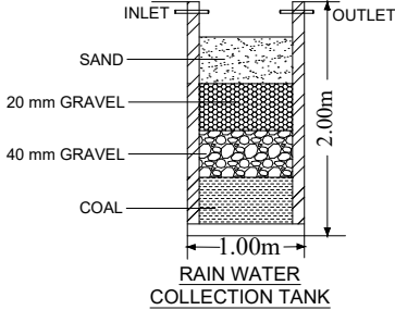
RAIN WATER COLLECTION TANK
