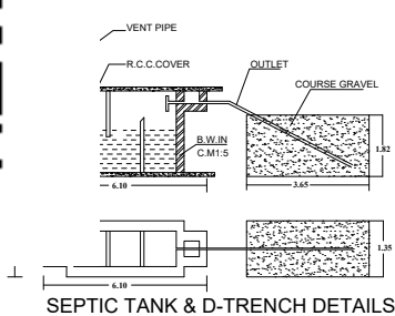
SEPTIC TANK & D-TRENCH DETAILS
