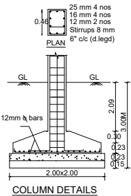
COLUMN DETAILS
