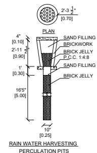
RAIN WATER HARVESTING PERCOLATION PITS
