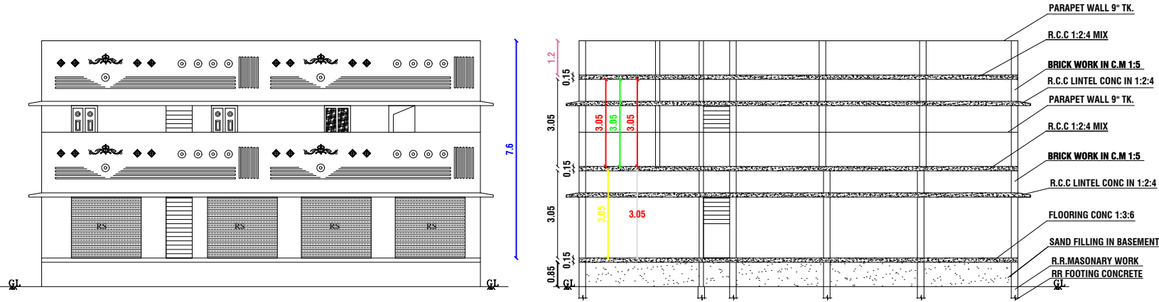
SECTION "A-A"
