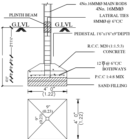
FOUNDATION DETAIL
