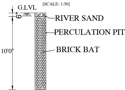
PERCOLATION PIT
