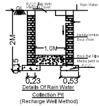
Details Of Rain Water Collection Pn (Recharge Well Method)
