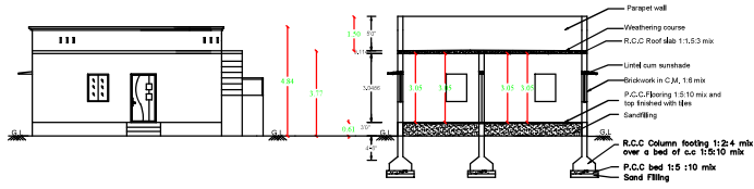
FRONT ELEVATION
