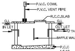
SEC. OF SEPTIC TANK
