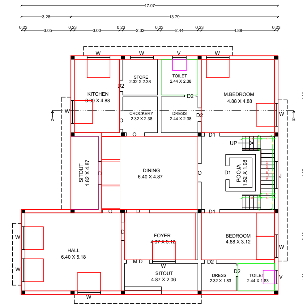
GROUND FLOOR
