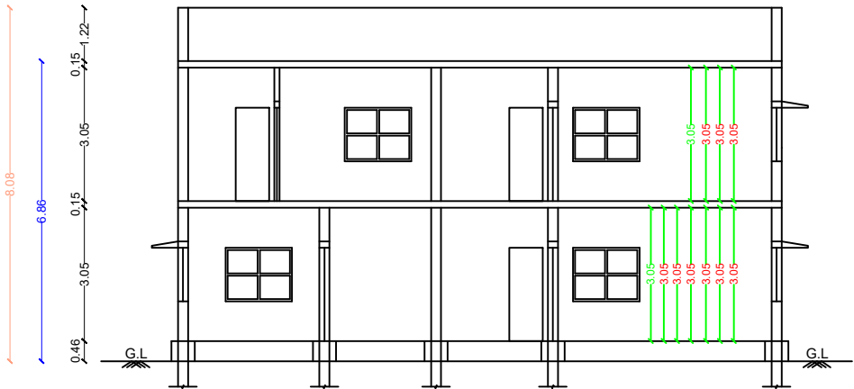
SECTION"A-B"
