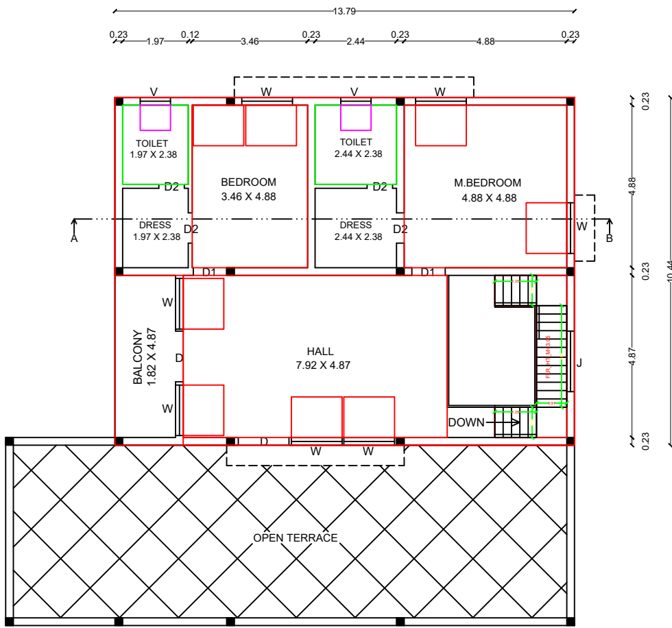
FIRST FLOOR
