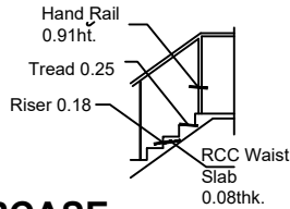
STAIRCASE DETAILS
