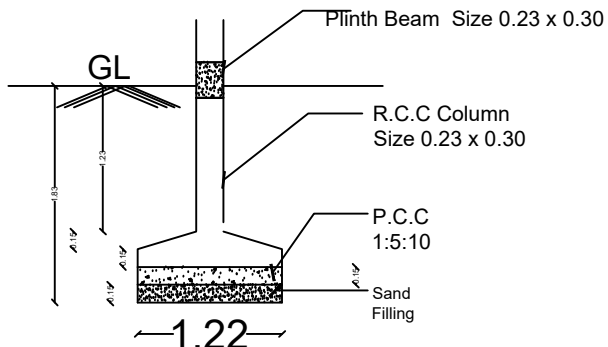
FOUNDATION DETAILS
