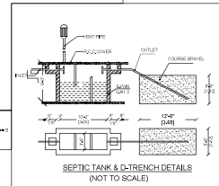
SEPTIC TANK & D-TRENCH DETAILS
