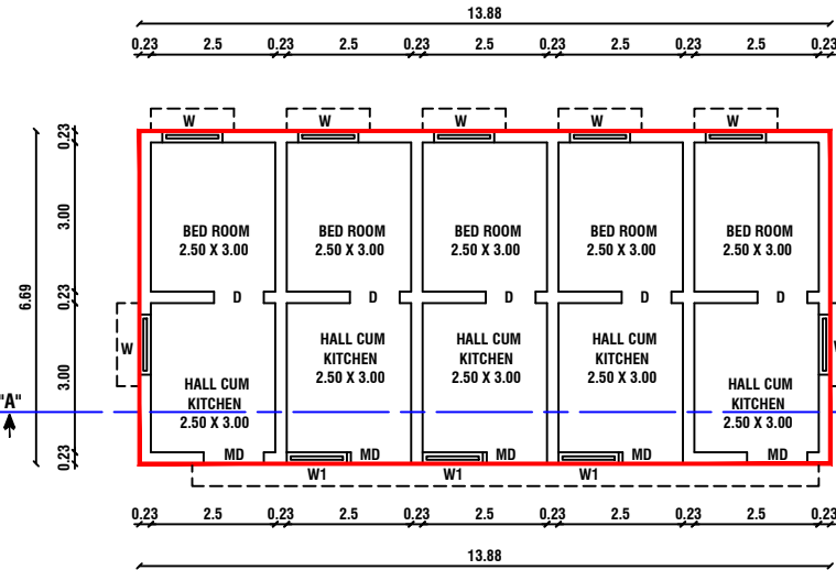
FLOOR GROUND
