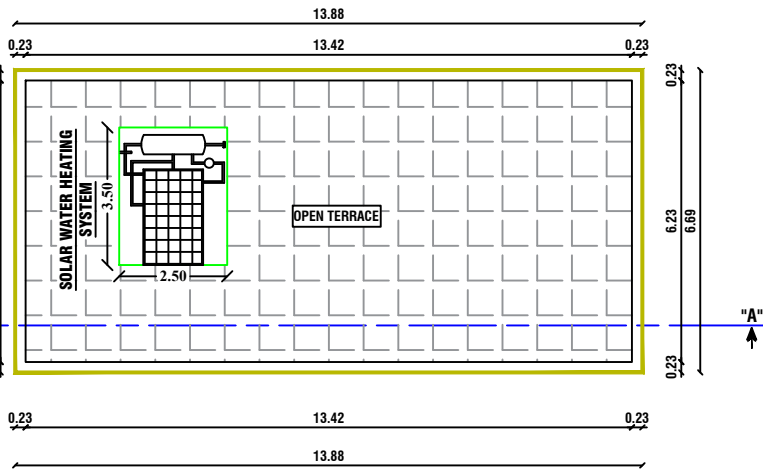
FLOOR-TERRACE
