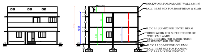
FRONT ELEVATION
