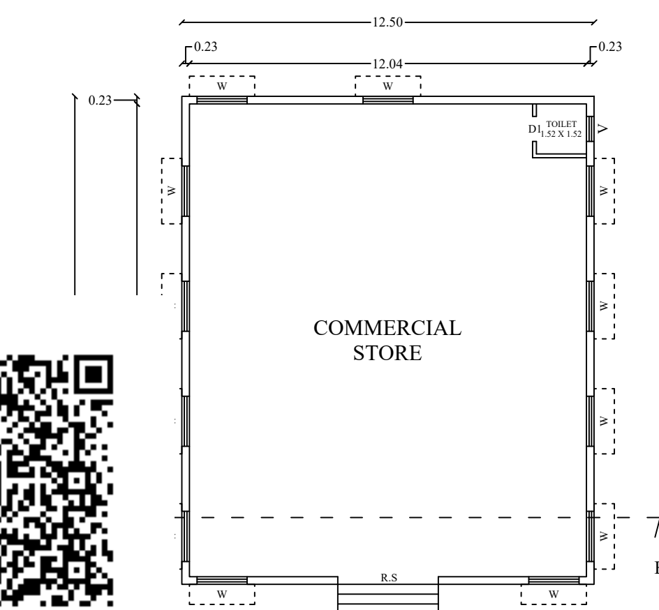
GROUND FLOOR
