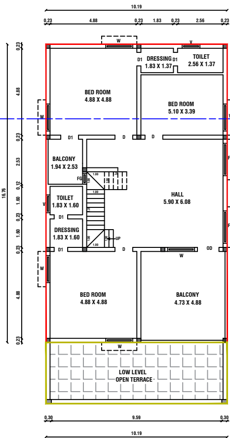
FLOOR FIRST
