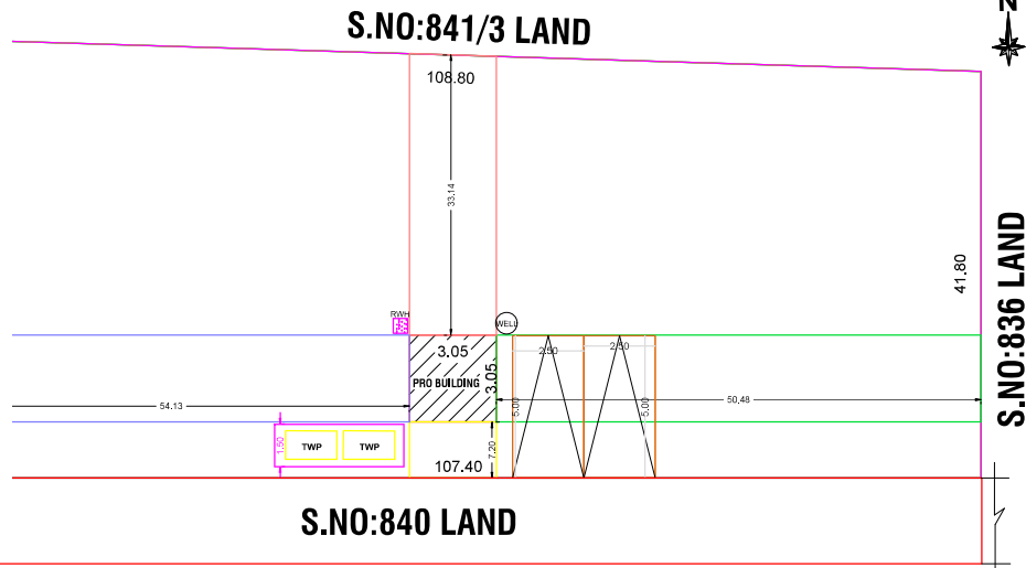
SITE PLAN
