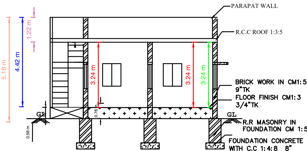
SECTION " AB "
