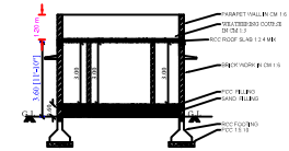
SECTION - "SR"
