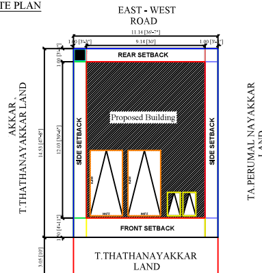
SITE PLAN
