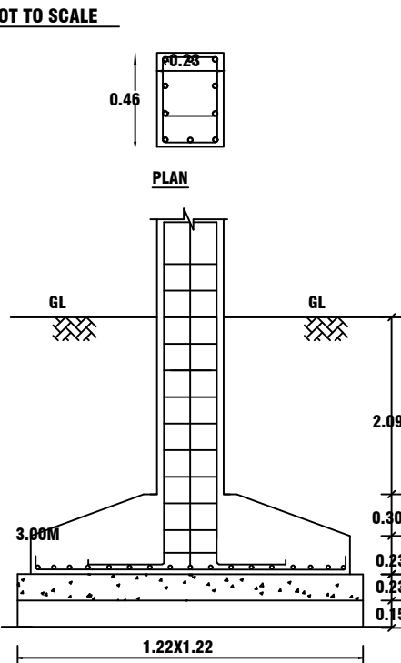
COLUMN DETAILS
