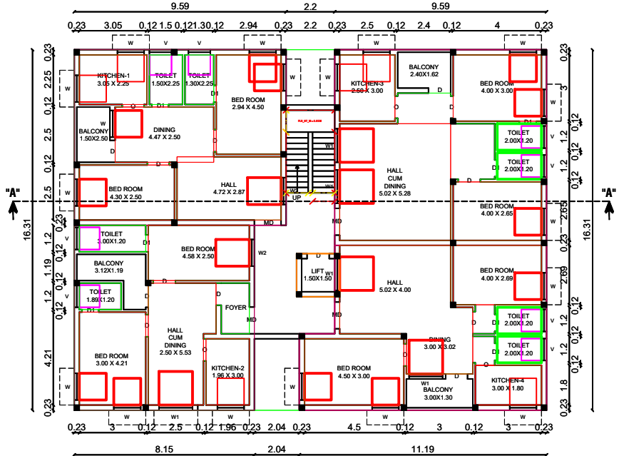
FLOOR - FIRST & SECOND PRO. FIRST & SECOND FLOOR PLAN
