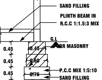
RR MASONRY DETAILS
