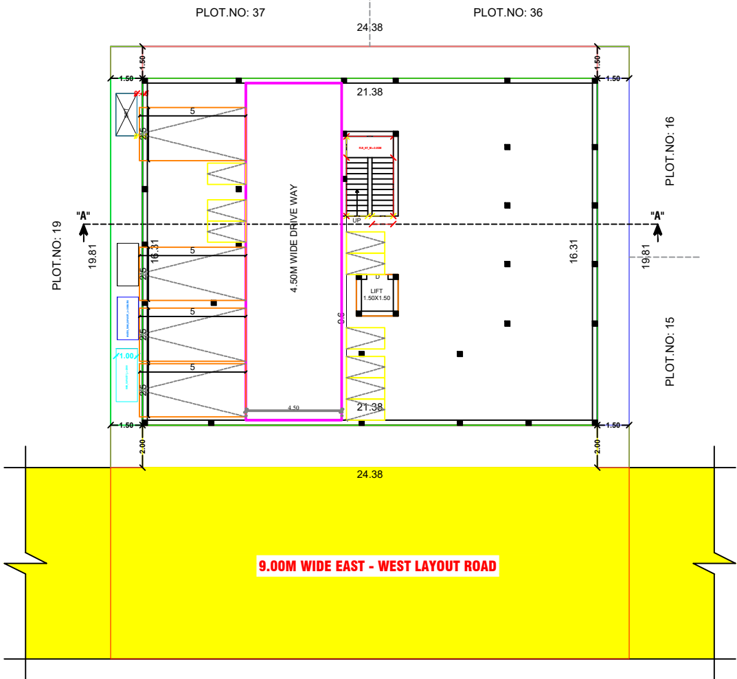
SITE PLAN AND STILT FLOOR
