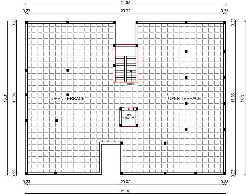
FLOOR - TERRACE PRO. TERRACE FLOOR PLAN
