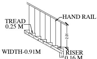
STAIRCASE DETAILS
