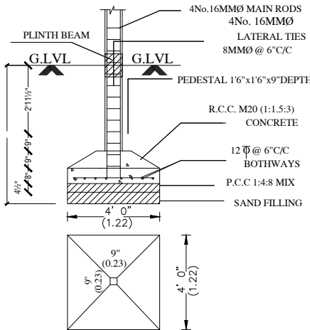
FOUNDATION DETAIL
