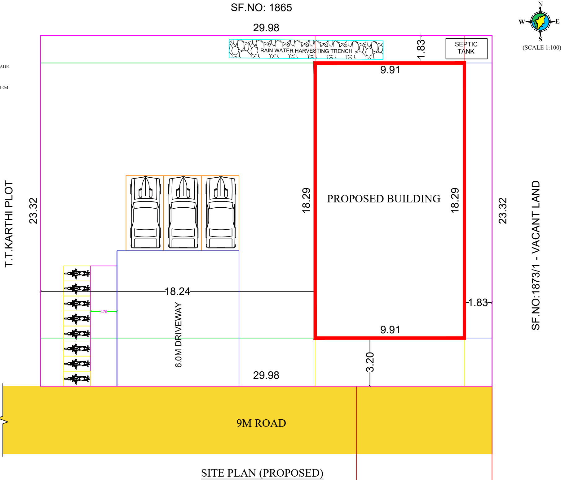
SITE PLAN (PROPOSED)
