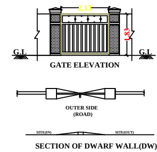
GATE ELEVATION SECTION OF DWARF WALL (DW)
