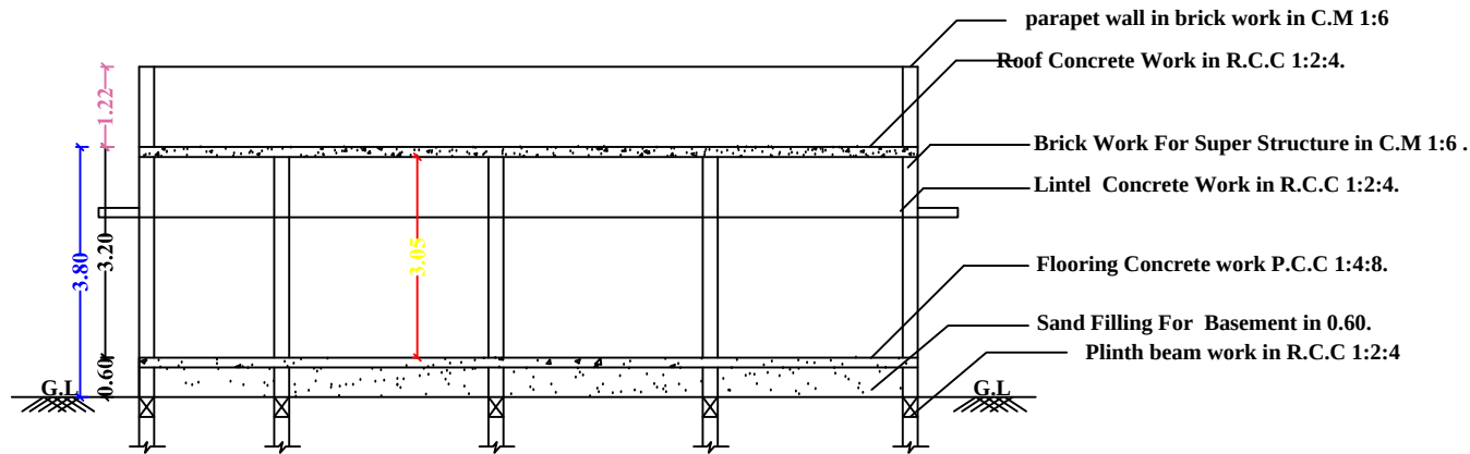
SECTION-AB
