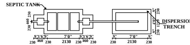
PLAN SEPTIC TANK DETAILS.
