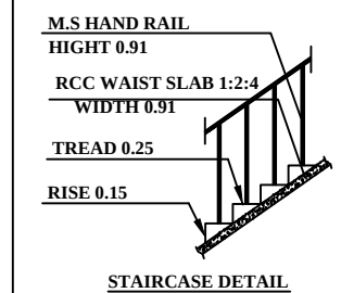
STAIRCASE DETAIL
