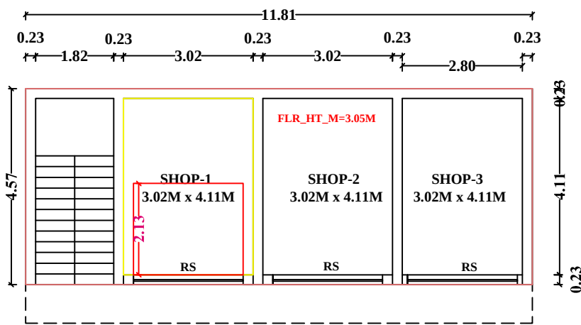
FLOOR-0 PRO.GROUND FLOOR PLAN
