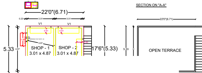
R PLAN
