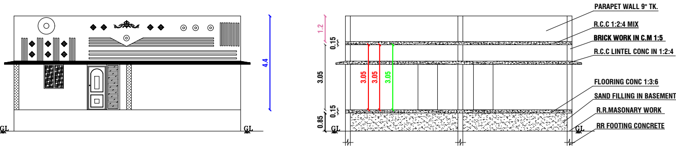
FRONT ELEVATION
