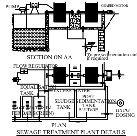
PLAN SEWAGE TREATMENT PLANT DETAILS
