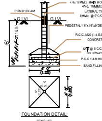
FOUNDATION DETAIL
