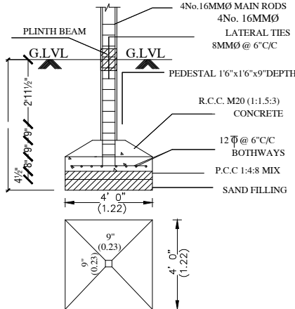
FOUNDATION DETAIL
