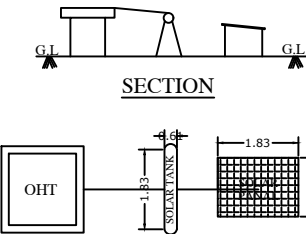
SOLAR SYSTEM PLAN
