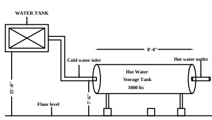
SOLAR WATER HEATER DETAILS (NOT TO SCALE)
