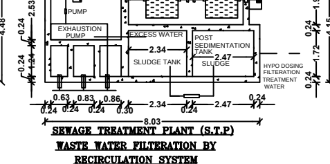
SEWAGE TREATMENT PLANT (S.T.P.) WASTE WATER FILTRATION BY RECIRCULATION SYSTEM G.O(MS) No.138 DT:11.10.02
