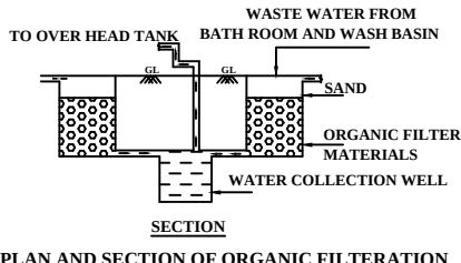
PLAN AND SECTION OF ORGANIC FILTRATION SUMP WITH COLLECTION WELL
