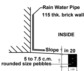
INSIDE Slope 1 in 20 5 to 7.5 c.m. rounded size pebbles Percolation pit
