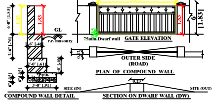
COMPOUND WALL DETAIL
