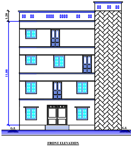
FRONT ELEVATION
