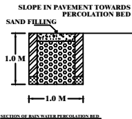
SECTION OF RAIN WATER PERCOLATION BED
