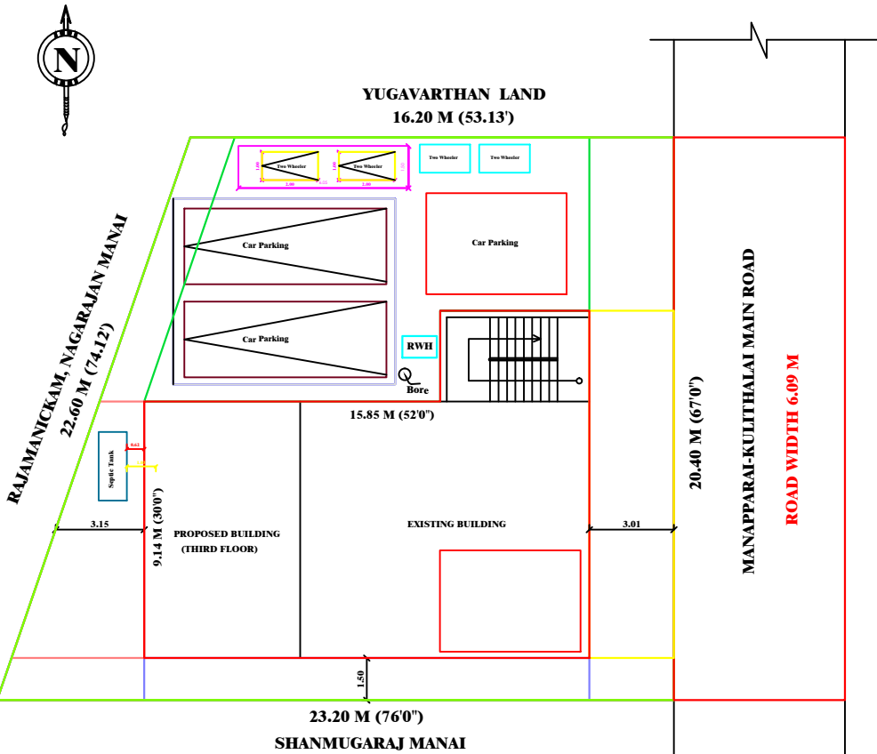
SITE PLAN
