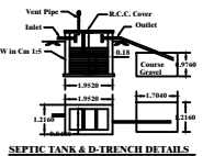
SEPTIC TANK & D-TRENCH DETAILS
