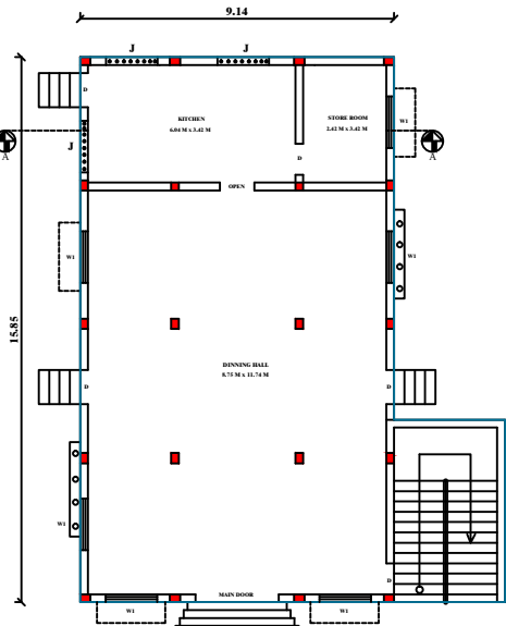
EXISTING STILL (OR) GROUND FLOOR PLAN
