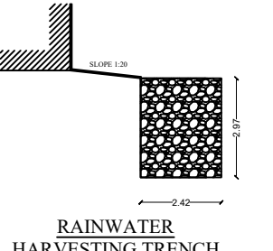
RAINWATER HARVESTING TRENCH
