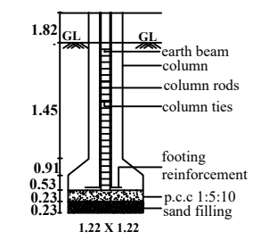
FOUNDATION DETAILS
