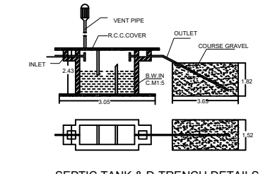
SEPTIC TANK & D-TRENCH DETAILS
