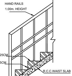
SECTION ON STAIRCASE
