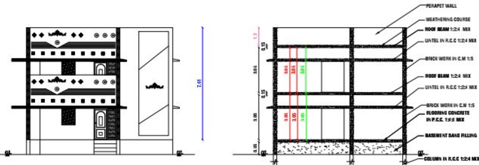
FRONT ELEVATION
