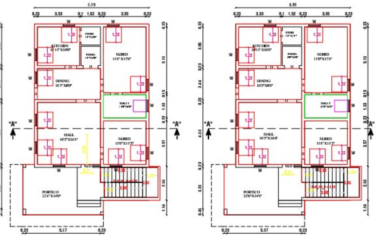
GROUND FLOOR
