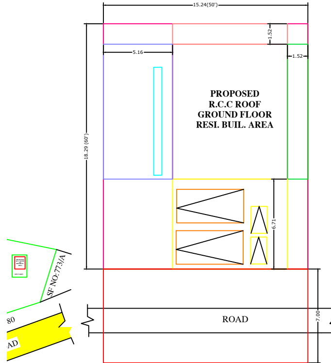
SITE TAKEN PLAN
