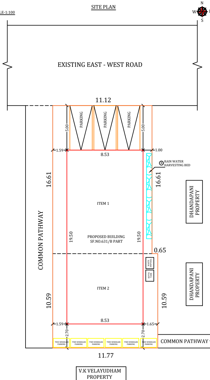
SITE PLAN
