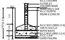
FOUNDATION DETAILS
