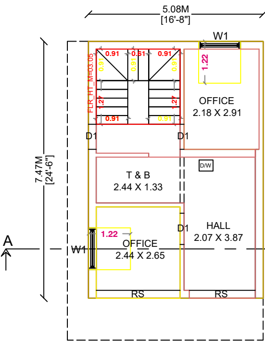
PROPOSED GROUND FLOOR PLAN (COMMERCIAL)
