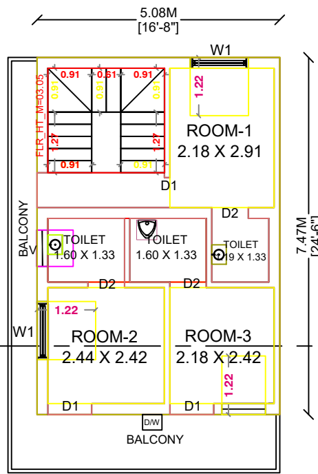
PROPOSED FIRST FLOOR PLAN (COMMERCIAL)
