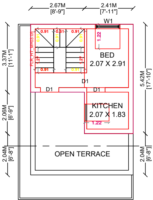
PROPOSED SECOND FLOOR PLAN (RESIDENTIAL)
