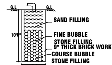
SECTION ON RAIN WATER COLLECTION TANK
