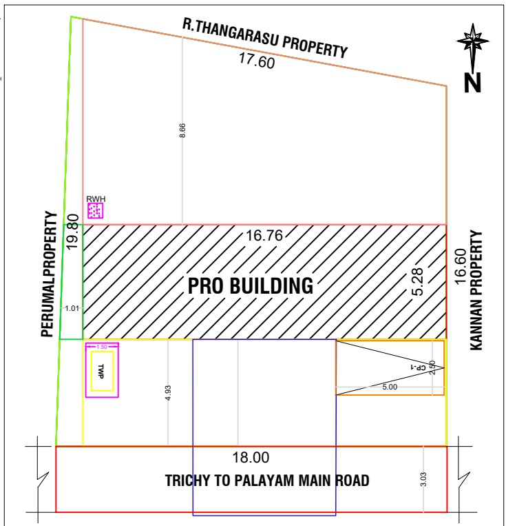
SITE PLAN
