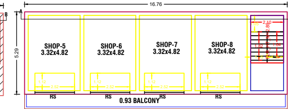
PRO.,FIRST FLOOR PLAN
