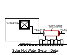
Solar Hot Water System Detail
