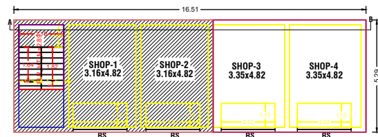
EXISTING.,GROUND FLOOR PLAN ADDITIONAL.,GROUND FLOOR PLAN
