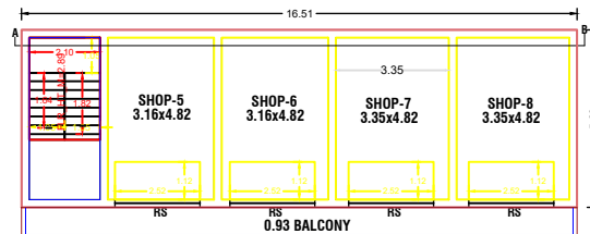
PRO.,FIRST FLOOR PLAN
